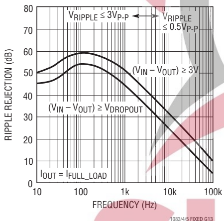
LT1083/4/5-12 Ripple Rejection
